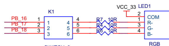
SWITCH_3
