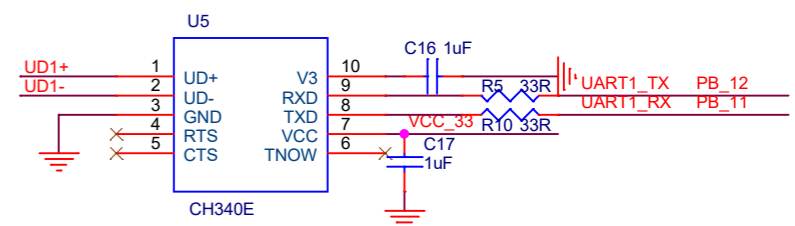
USB to Uart1
