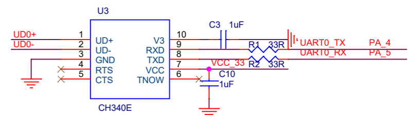
USB to Uart0
