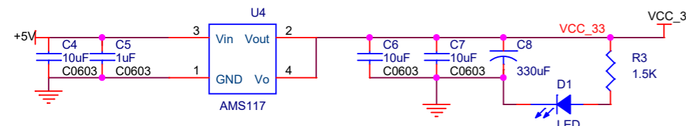
LDO power supply
