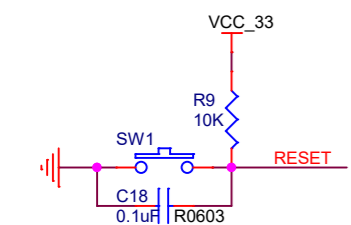
RESET key
