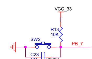
USER key
