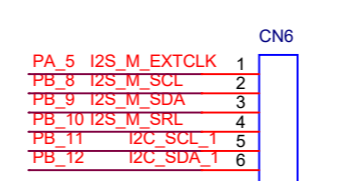
I2S_M&I2C
